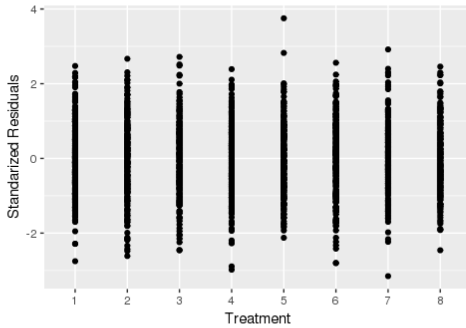
Standardized Residuals vs. Treatment
